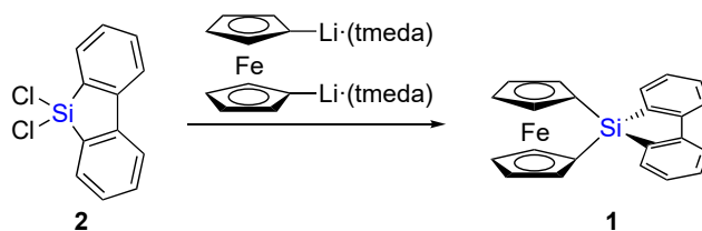
Scheme 1. Synthesis of sila[1]ferrocenophane 1 .
